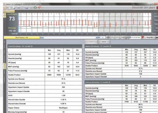
STATISTICS VIEW
